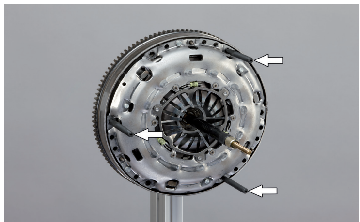
Fig. 2: Stud bolts for holding the spindle carrier
