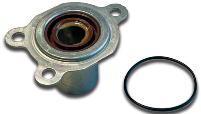
Figure 1: Guide tube 414 002410 with separate sealing ring
