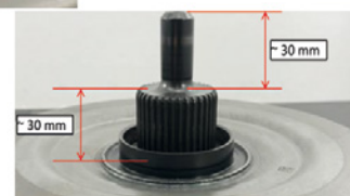
Figure 3: Modified dimensions of the gearing and the guide pin
