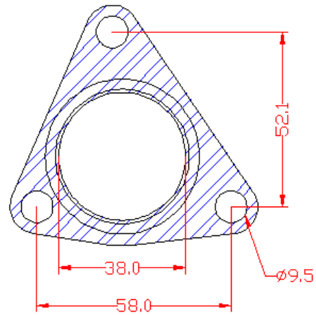
Gasket dimensions
