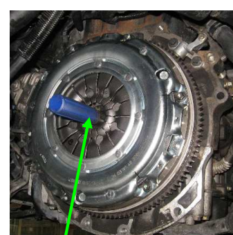
Centering tool
