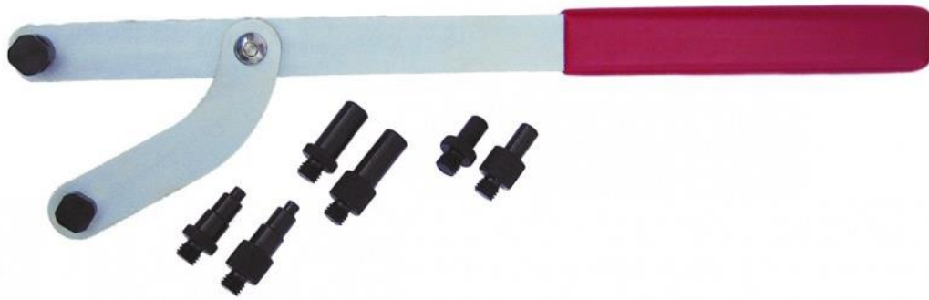
7468-10022 – GAT4844 – Sprocket Holding Tool
