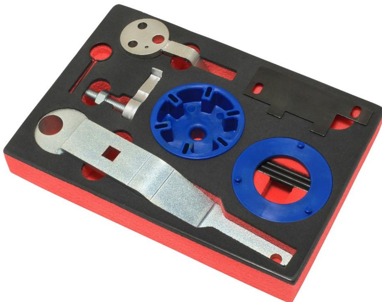
7468-11326 – GAT5105 – Engine Setting and Locking Tool Kit
