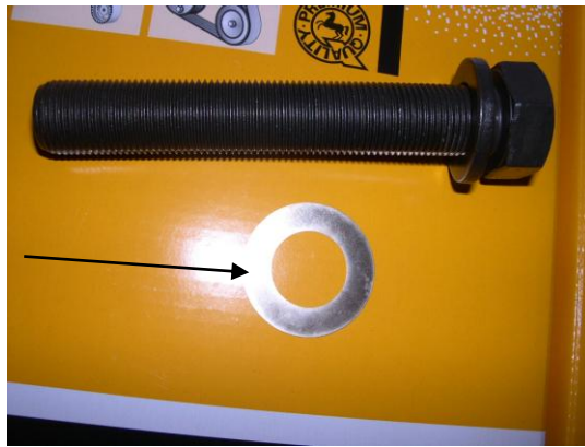
Fig. 1 Washer
