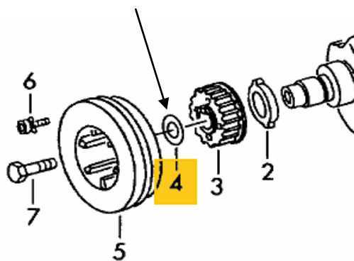
Fig. 2 Installed position
