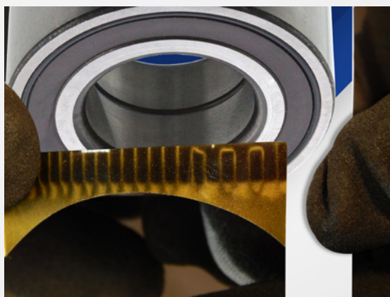
Example of a faulty retractor using a magnetic test card
