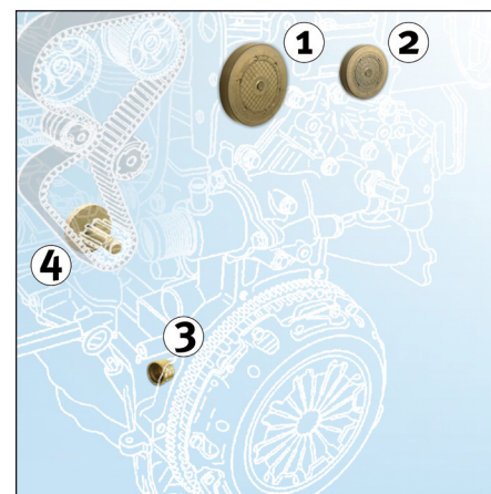
Figure 2: Installation position
