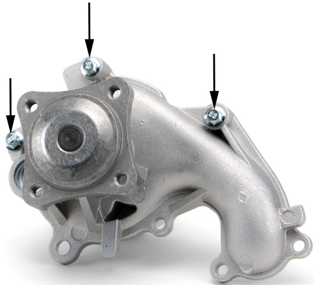
Fig. 2: Modified mounting points of the coolant pump
