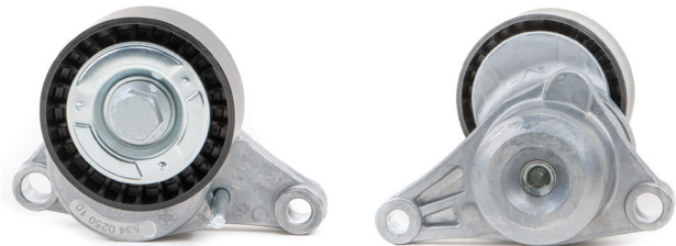
Figure 2: New design
