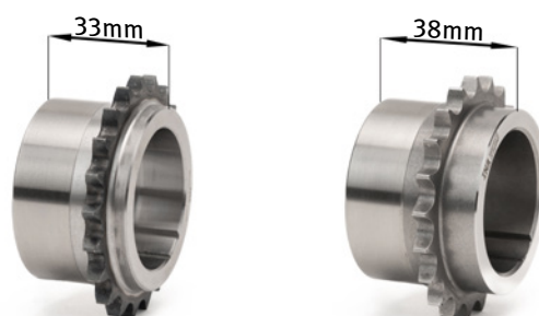
Figure 1: Crankshaft gear 554 0996 10 with a length of 33 mm (left) is part of timing chain kit 559 1780 30. Crankshaft gear 554 0101 10 with a length of 38 mm (right) is part of timing chain kit 559 1780 31
