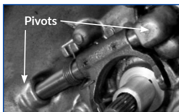
Worn or Seized Release mechanism pivots
