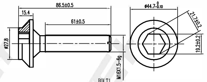
BOLT1 1PCS BLACK
