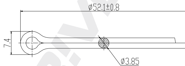
Cotter 1pcs
