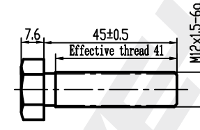
BOLT 2pcs Galvanizing
