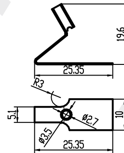
Spring 1pcs Brass
