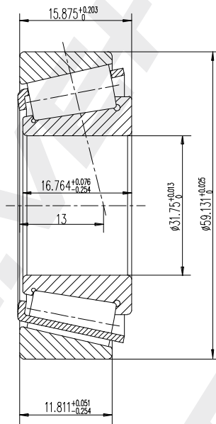
BEARING2
