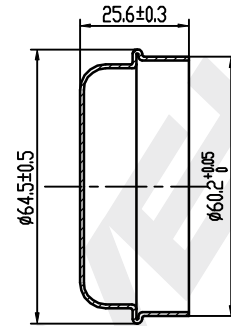
CAP 1pcs Galvanizing
