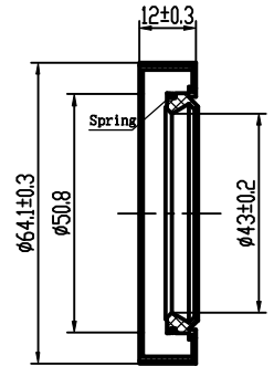
SEAL 1pcs
