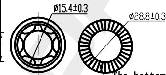
BOLT 1pcs Dacromet
