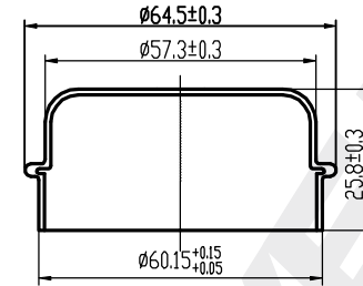
CAP 1pcs Galvanizing
