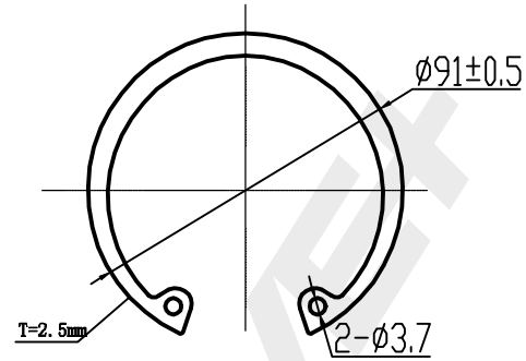
Circlip 1pcs black
