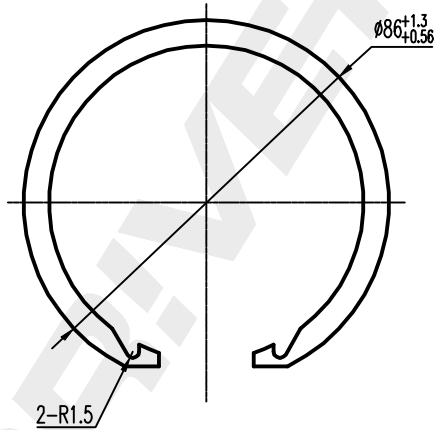
Circlip 1pcs black
