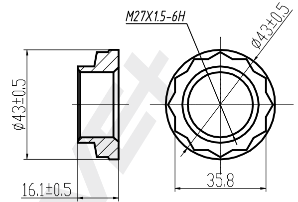
NUT 1pcs Galvanizing
