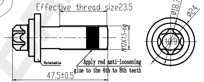
BOLT 4pcs Dacromet
