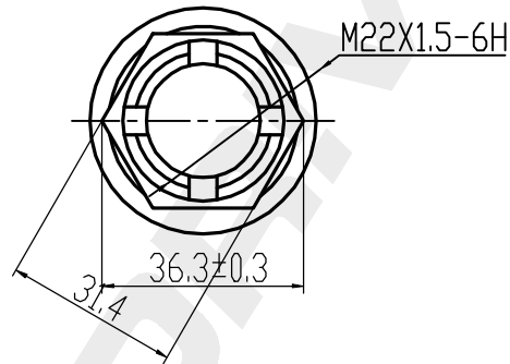
NUT 1pcs Galvanizing
