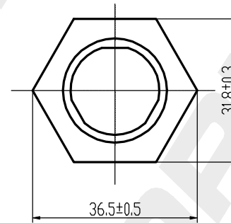
NUT 1pcs Yellow zinc plating
