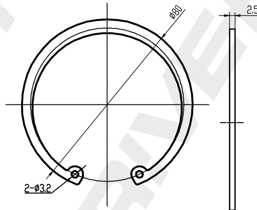
Circlip 1pcs black
