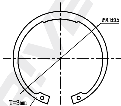
Circlip 1pcs black
