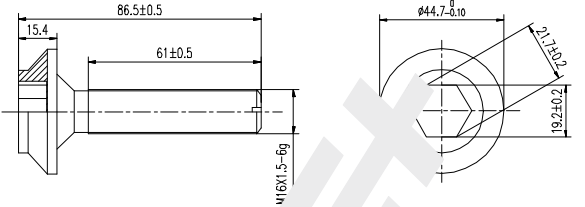
Bolt 163-D-001 1PCS Black
